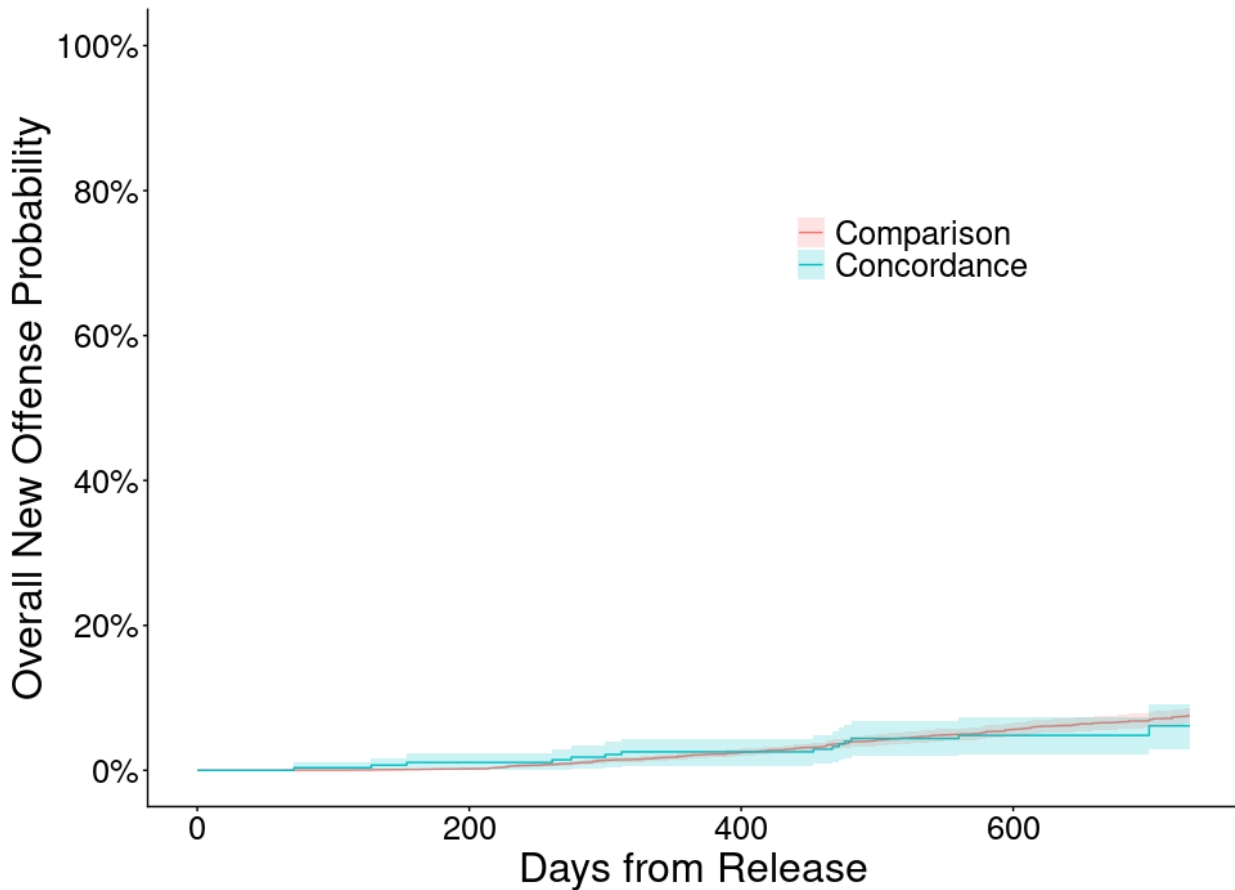
Figure 3. Probability of New Offense Over Time by Group
